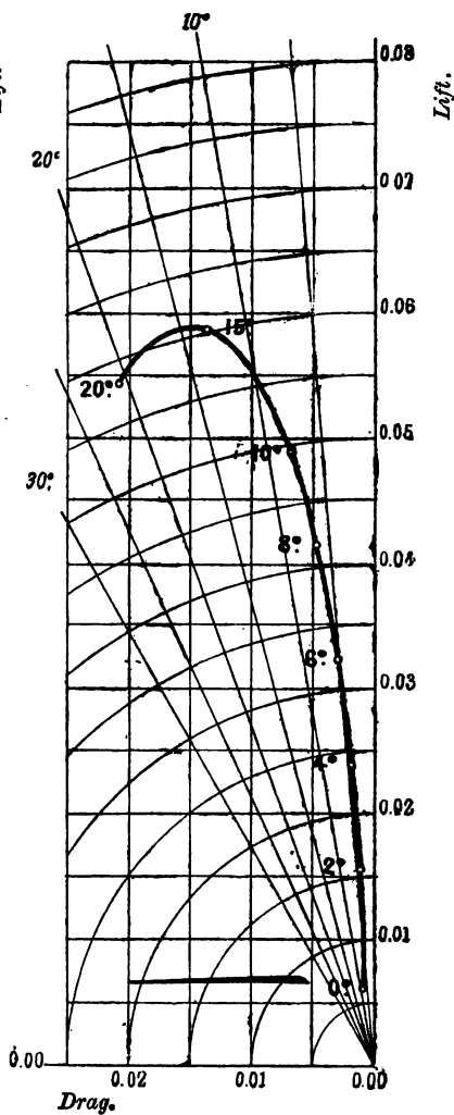
FIG. 2.—Maurice Farman plane.
